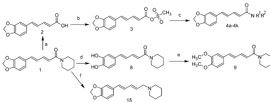
Scheme 1. (a) KOH (b) MeSO_2Cl , Et_3N , CH_2Cl_2 , 0^\circ C 45 min (c) R^1R^2NH , 0^\circ C 1 h, rt 2 h (d) BBr_3 in CH_2Cl_2 rt 48 h (e) DMSO/KOH, CH_3I , nitrogen atmosphere, 30 min (f) NaBH_4/I_2 , THF, 0^\circ C nitrogen atmosphere, 48 h.
