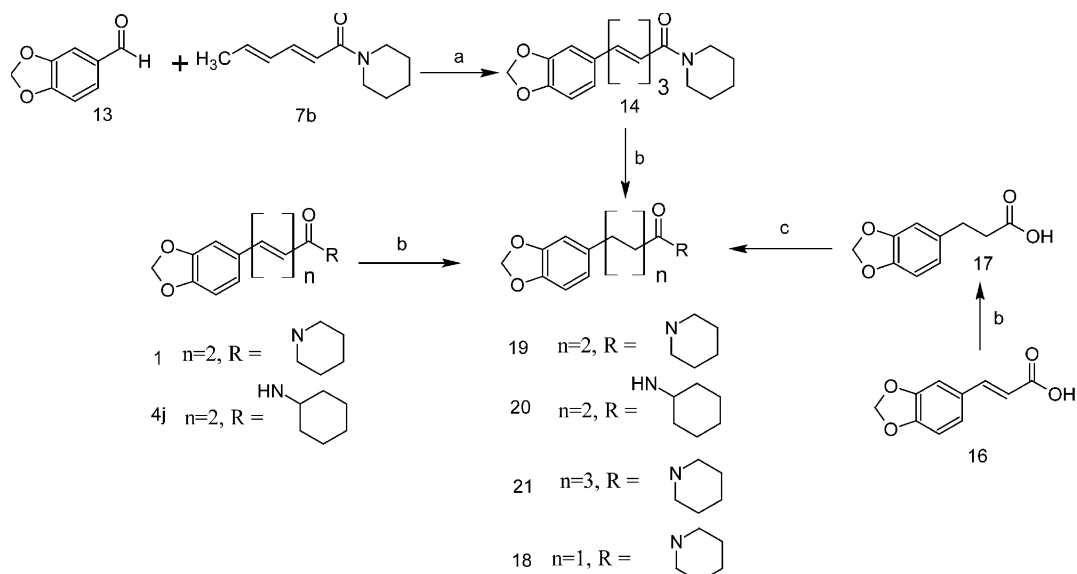
Scheme 2. (a) Aliquat 336, K_2CO_3/NaH , toluene, 90^\circ C 6 h (b) H_2 , Pd-C (c) MeSO_2Cl , Et_3N , CH_2Cl_2 , 0^\circ C 45 min, RNH , 0^\circ C 1 h, rt 1 h.
